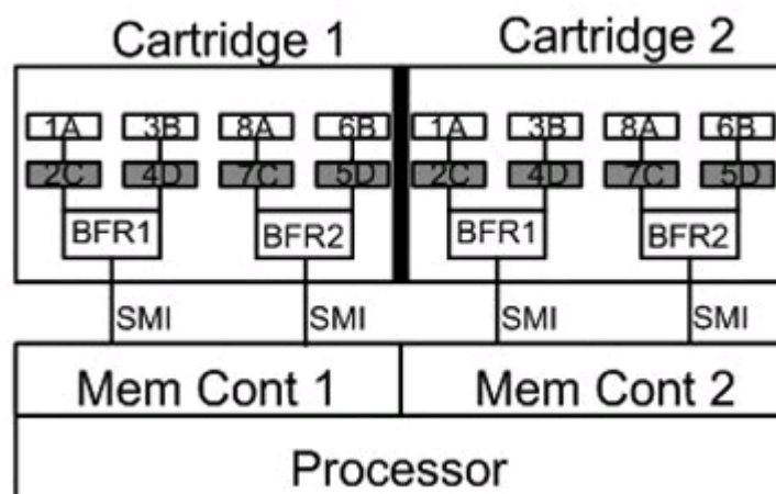
Figure 1 Processor/Memory interconnect
